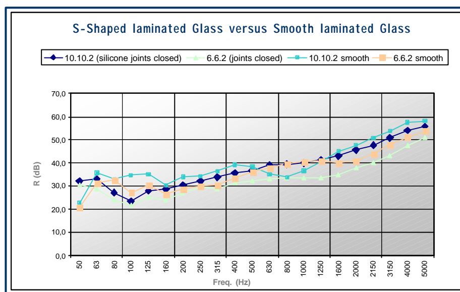
Figure 5 – S-Shaped glass TL values (dB) versus Smooth glass TL values (dB) (both laminated)
