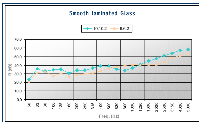
Figure 4 – Smooth laminated glass TL values (dB)
