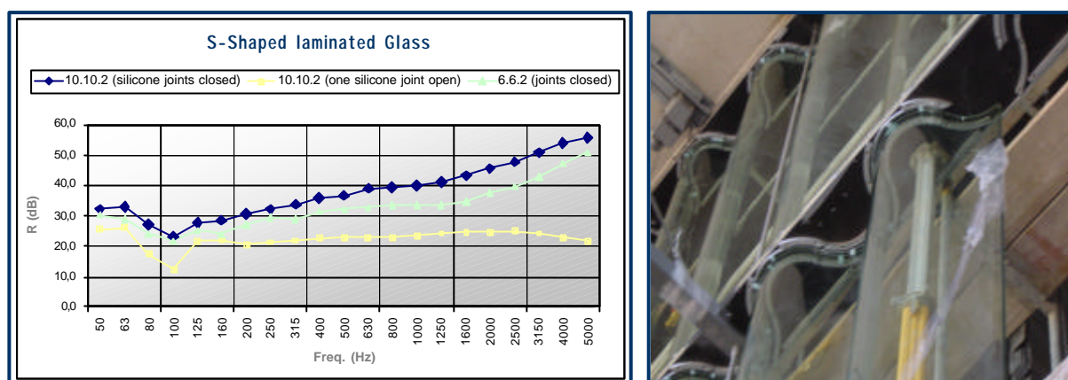
Figure 3 – S-Shaped laminated glass TL values (dB)
