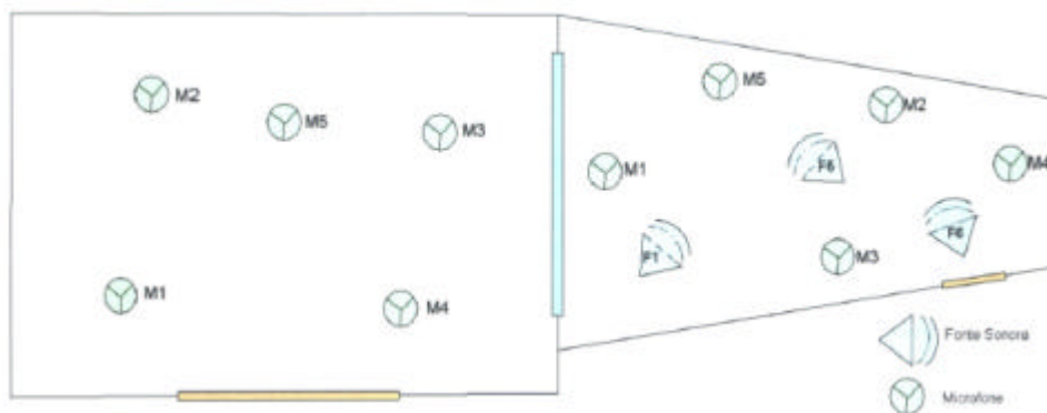
Figure 3 – Sound source and measuring points positions in the sound transmission rooms (no scale)
