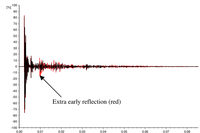
Figure 8: Overlay of two IR's close to a wall: curtains close (black) and one curtain partly opened (red)
