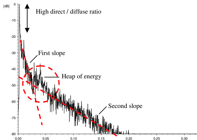
Figure 9: ETC of IR measured in front of closed tent
