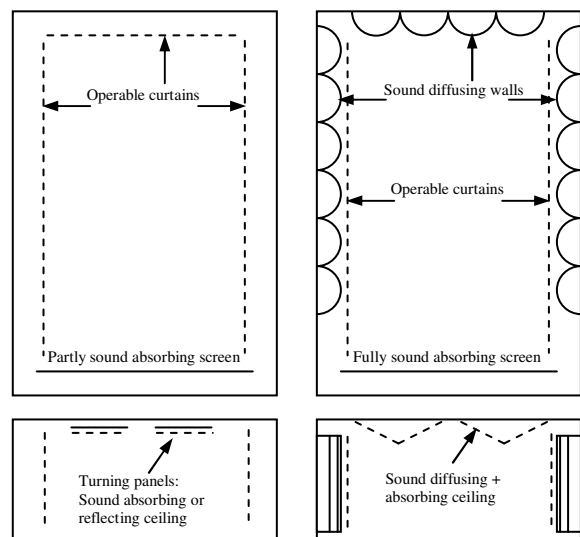
Figure 2: Schematic acoustic design in floor plans (upper drawings) and sections (lower drawings) of the typical studio (left) and the studio with good reputation (right)
