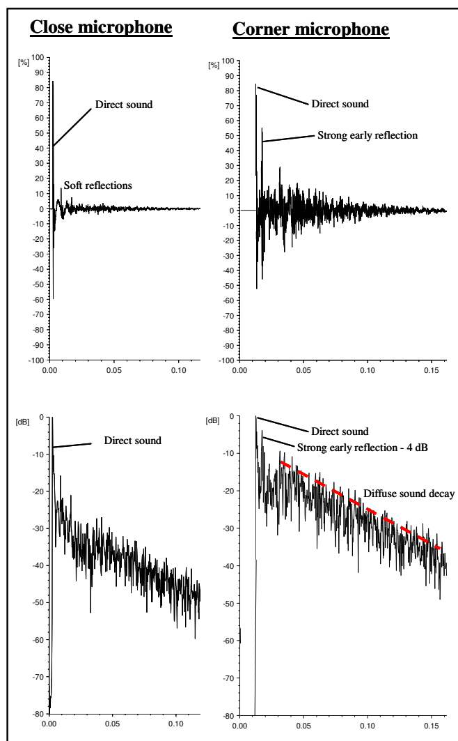
Figure 6: Impulse responses (upper graphs) and energy time curves (lower graphs) of close (left) and corner microphone (right)
