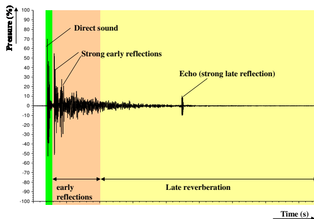
Figure 4: Typical acoustical impulse response
