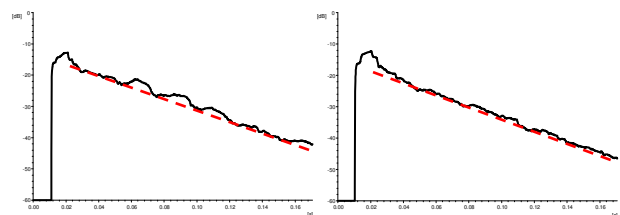
Figure 7: Energy time curves (10 ms RMS average) with trend lines in red of typical studio (left) and studio with good reputation (right).
