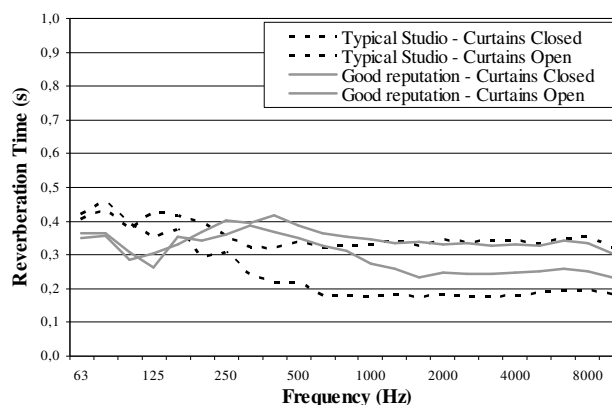
Figure 5: Reverberation time T_{30} versus frequency for both studios with and without curtains.
